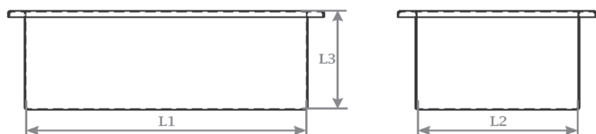
Welded tank
